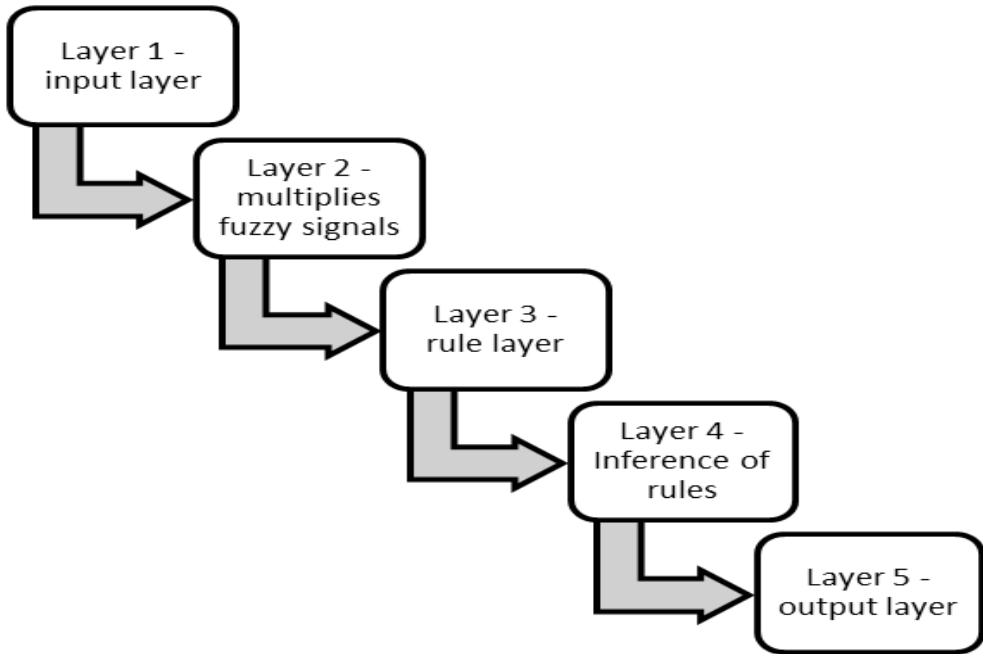
Figure 1. ANFIS layers
